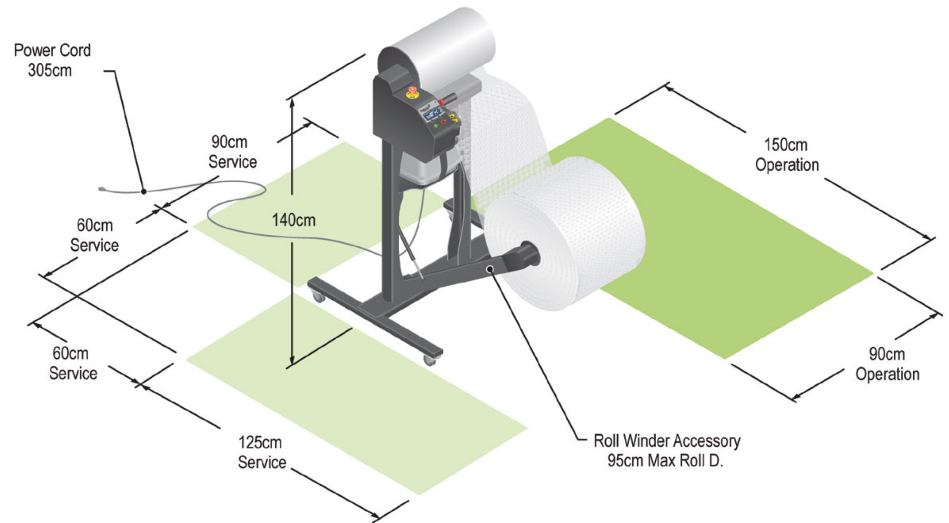
System Set-up - Stand with Roll Winder Version
